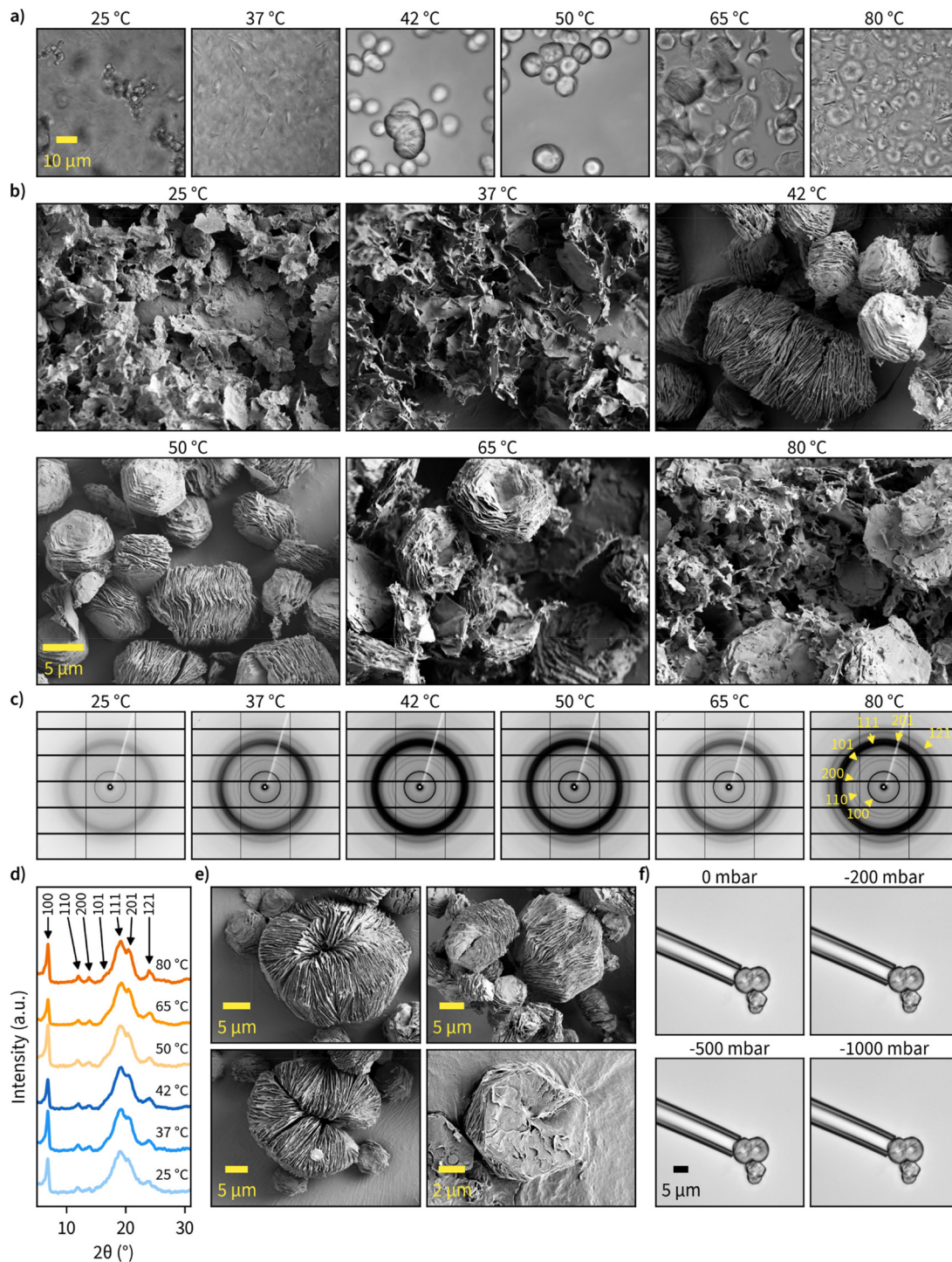
Fig. 2 Effect of reaction temperature on hexagonal \beta -1,3-D-glucan microparticle assembly and crystallinity. (a) Transmitted light images obtained with a confocal microscope of never-dried \beta -1,3-D-glucan particles synthesized at different temperatures. (b) SEM images of dried \beta -1,3-D-glucan particles synthesized at different reaction temperatures. (c) 2D synchrotron wide-angle X-ray scattering (WAXS) patterns of dried \beta -1,3-D-glucans prepared at different temperatures ( \lambda = 0.82656 Å). Yellow arrows annotate the major diffraction rings corresponding to triple-helical \beta -1,3-D-glucan, and the corresponding Miller indices. (d) 1D WAXS profiles with major diffraction peaks indicated with arrows ( \lambda = 1.5418 Å). (e) SEM images of different types of hexagonal assemblies observed for \beta -1,3-D-glucans synthesized at 50 °C. (f) Micropipette aspiration of hexagonal particles synthesized at 50 °C performed with a micropipette with a tip diameter of 10 \mu\text{m} and pressure ranging from 0 to -1000 mbar.
