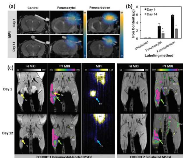
Fig. 16 The in vivo tracking of MSCs with MPI. (a) In vivo MPI images at days 1 and 14 following the implantation of ferumoxytol- or ferucarbotran-labelled therapeutic MSCs, or unlabelled MSCs as a control, in calvarial defects of experimental mouse subjects. (b) Iron content in the calvarial defects at days 1 and 14 following implantation of the differently labelled MSCs, as calculated from the MPI signals. Reproduced with permission of Springer Nature, from ref. 11; permission conveyed through Copyright Clearance Center, Inc. (c) In vivo 1 H/ 19 F MRI and MPI images at days 1 and 12 following the implantation of ferumoxytol-labelled therapeutic MSCs, and unlabelled MSCs as a control, in experimental mouse subjects. Reproduced from ref. 19 with permission from the Multidisciplinary Digital Publishing Institute. This is an open access article distributed under the terms of the CC BY-NC-ND License ( https://creativecommons.org/licenses/by-nc-nd/4.0/ ). Copyright 2019, the authors. Article can be found at: https://www.ncbi.nlm.nih.gov/pmc/articles/PMC6935990/ . No changes were made to the original figure.
