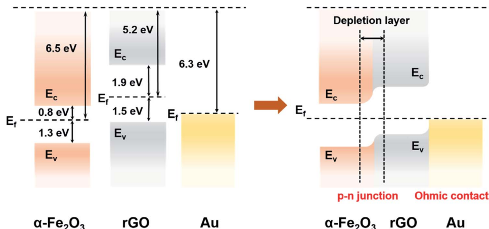
Fig. 3 Schematic of the band level diagram of the Au ND-ODT/ \alpha\text{-Fe}_2\text{O}_3 /rGO composite.
