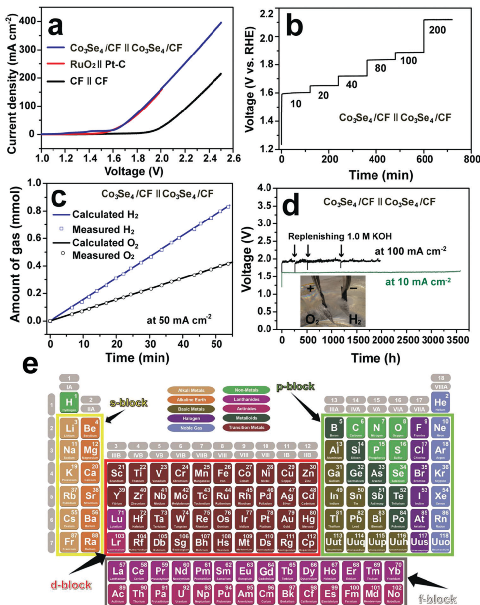
Fig. 5 Overall water splitting performance of the two-electrode electrolyser. (a) Polarization curves of \text{Co}_3\text{Se}_4/\text{CF} , CF and \text{RuO}_2(+) \parallel \text{Pt-C}(-) supported on CF. (b) Multi-step CP curve of the \text{Co}_3\text{Se}_4/\text{CF} electrolyser at varying current densities. (c) Gas yield of \text{H}_2 and \text{O}_2 evolved over the \text{Co}_3\text{Se}_4/\text{CF} electrodes as a function of time at 50 \text{ mA cm}^{-2} . (d) Long-term stability CP test of the \text{Co}_3\text{Se}_4/\text{CF} electrolyser at 10 and 100 \text{ mA cm}^{-2} . Inset is a photograph showing the gas bubbling of \text{H}_2 from the cathode and \text{O}_2 from the anode at 100 \text{ mA cm}^{-2} . All experiments were conducted in 1.0 \text{ M KOH} at room temperature. The polarization and CP curves are shown without iR correction. (a–d) Reproduced with permission from ref. 164. Copyright 2017, John Wiley and Sons, Inc. (e) The periodic table of s-, p-, d-, and f-block elements. Reproduced from ref. 205 with permission from John Wiley and Sons, Inc. under the Creative Commons CC BY license.
