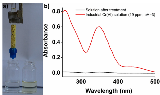
Fig. 7 (a) \text{Cr(VI)} industrial waste sorption by the column filled with BUT-MOF/calcium alginate beads (initial \text{Cr(VI)} concentration = 19 ppm, pH = 3, 480 mg of sorbent) and (b) UV-Vis spectra of the \text{Cr(VI)} industrial waste solution before and after treatment.
