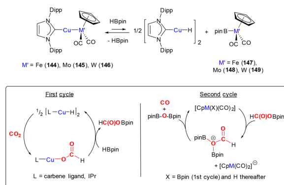
Scheme 43 Mechanism for the 2-electron reduction of CO 2 to CO catalysed by heterobimetallic complexes [(NHC)Cu–ML n ] {ML n = [FeCp(CO) 2 ], [WCp(CO) 3 ], [MoCp(CO) 3 ]}.
