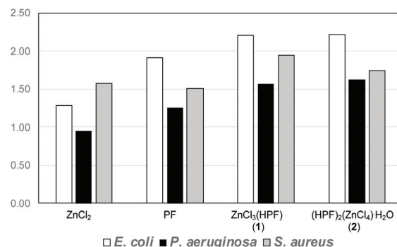
Fig. 15 Fold antimicrobial activity of proflavine, ZnCl 3 (HPF) and [HPF] 2 [ZnCl 4 ]·H 2 O compared to the activity of AgNO 3 (the value of 1.00 is equal efficacy as silver nitrate). Reproduced from ref. 69 with permission from the Royal Society of Chemistry.
