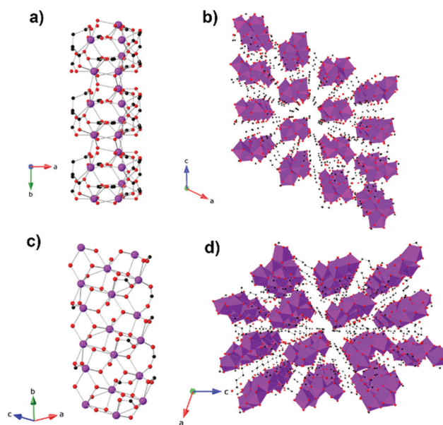
Fig. 12 (a) Crystal structure of \text{Gd}_2(\text{OH})_2(\text{suc})_2(\text{H}_2\text{O}) \cdot 2\text{H}_2\text{O} with a two-rail Gd–OH ladder parallel to the b -axis and (b) the packing of the ladders on the ac -plane. (c) Crystal structure of \text{Gd}_6(\text{OH})_8(\text{suc})_5(\text{H}_2\text{O})_2 \cdot 4\text{H}_2\text{O} showing the three-rail Gd–OH ladder parallel to the b -axis and (d) the packing of the three-rail ladders on the ac -plane. Colour codes: Gd: purple, C: black, O: red. Hydrogens are omitted for clarity.
