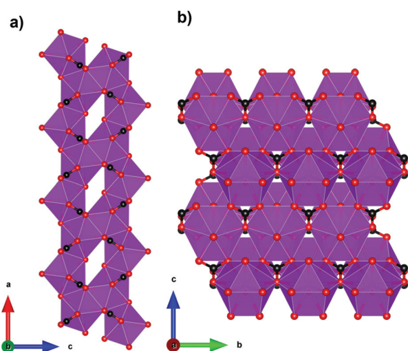
Fig. 5 (a) Crystal structure of GdOHCO 3 with face-sharing GdO 10 polyhedra forming zig-zag chains along the a -axis and (b) packing of the distorted triangular lattice along the bc -plane. Colour codes: Gd: purple, C: black, O: red. The hydrogen atoms have been omitted for clarity.
