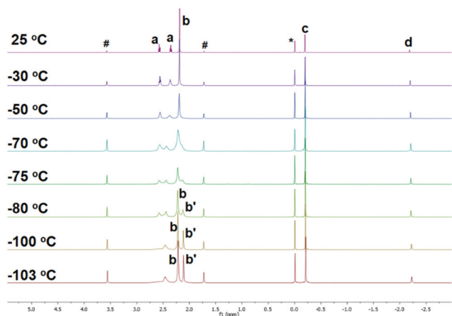
Fig. 2 Variable temperature (VT) ^1\text{H} NMR of complex 1 in d_8\text{-THF} . (a): \text{NCH}_2\text{CH}_2 ; b and b': \text{NMe}_2 ; c: \text{CH}_2\text{SiMe}_3 ; d: \text{CH}_2\text{SiMe}_3 ; *: \text{Me}_4\text{Si} ; #: d_8\text{-THF} .
