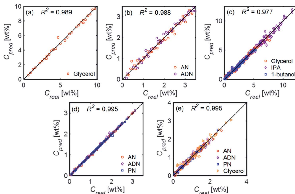
Fig. 12 Predicted ( C_{pred} ) compared to real ( C_{real} ) mass concentrations [wt%] for LR models on (a) 1-Gly, (b) 2-AN, (c) 3-Gly, (d) 3-AN, and (e) 4-AN mixture.
