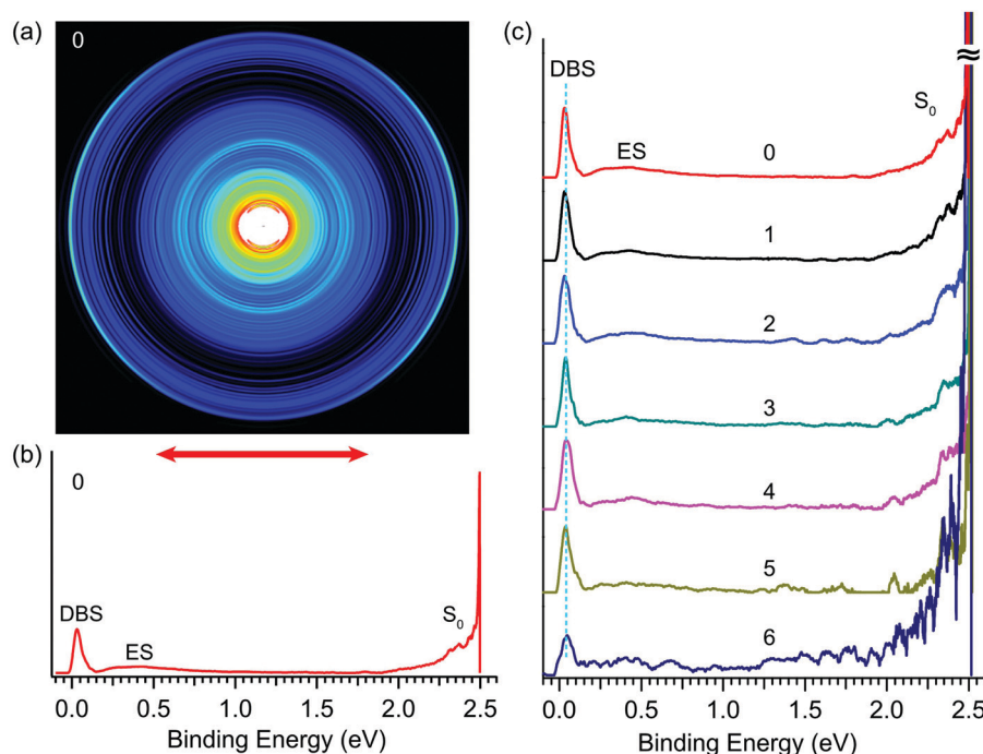
Fig. 5 Resonant two-photon photoelectron images and spectra of R -TFAE − at detachment wavelengths corresponding to peaks 0–6 shown in Fig. 4. (a) The photoelectron image at peak 0 (496.42 nm, 2.4975 eV); (b) the R2PD photoelectron spectrum inverted from the image in (a); the three observed features are labelled as DBS, ES, and S 0 ; (c) comparison of the seven R2PD photoelectron spectra, the peak numbers from Fig. 4 are indicated, see Table 2 for the wavelengths of peaks 1–6.
