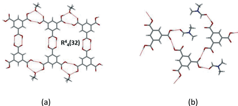
Fig. 7 (a) H_3btc \cdot EtOH solvate which shows typical layer formed in alcohol solvates with [ChemTemp]^{46} ; (b) disruption of the layer in the 2:1 H_3btc \cdot DMF solvate (XAVPOZ 47 ) (adapted from ref. 44).
