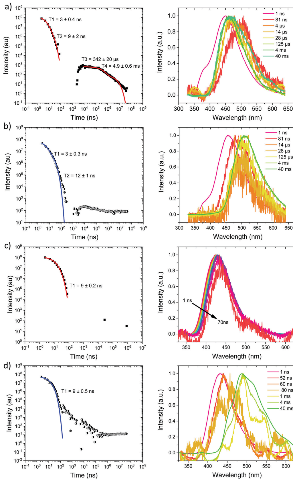
Fig. 5 Time-resolved spectroly integrated intensity decay (left) and representative time resolved spectra (right) of (a) \text{Ph}_2\text{TRZCzPhCz} , (a) 300 K and (b) 80 K; \text{Ph}_3\text{TRZCzPhCz} , (c) 300 K and, (d) 80 K in zeonex matrix. Spectral times given in ns, and decay fitting data included in the decay plots.
