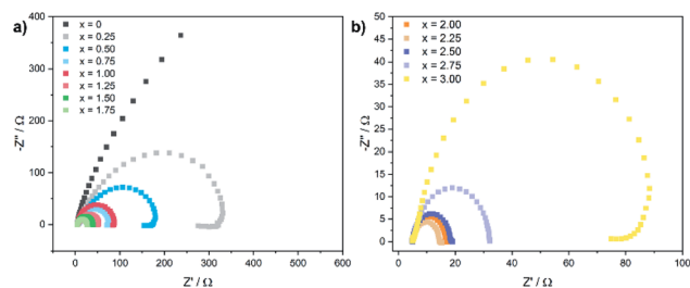
Fig. 5 Electrochemical impedance spectra (EIS) for (a) \text{Co}_x\text{Fe}_{3-x}\text{O}_4 ( x = 0-1.75 ) and (b) (\text{Co}_x/3\text{Fe}_{(1-x)/3})\text{O} ( x \geq 2 ) nanoparticles recorded at an overpotential of 550 mV.
