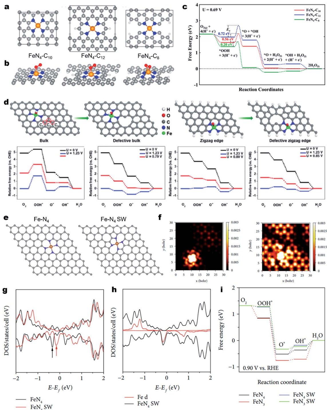
Fig. 6 Regulating the carbon skeleton geometry for enhancing the ORR activity. (a) Atomistic configuration of the Fe–N 4 moiety with different local carbon structures of Fe–N 4 –C 10 , Fe–N 4 –C 12 , and Fe–N 4 –C 8 and (b) corresponding O 2 adsorption configuration. (c) Calculated free energy diagrams for the ORR through an OOH dissociation pathway on the above three different active sites under a potential of 0.69 V in acidic medium. Reproduced with permission from ref. 160. Copyright (2017) American Chemical Society. (d) Schematic illustration of a bulk Fe–N 4 site, defective bulk Fe–N 4 site, zigzag Fe–N 4 site, and defective zigzag Fe–N 4 site and corresponding free energy diagram for the ORR. Reproduced with permission from ref. 163. Copyright (2019) Wiley-VCH. (e) Atomic models of Fe–N 4 and Fe–N 4 SW. (f) Simulated STM image (at a bias of –1.0 V) of normal Fe–N 4 doped graphene sheets (left) and Fe–N 4 SW doped graphene sheets (right). Density of states (DOS) of normal Fe–N 4 and Fe–N 4 SW-doped graphene sheets. (g) DOS of Fe–N 4 SW and (h) DOS of Fe 3d. (i) Free energy diagrams of ORR processes on normal Fe–N 4 , normal Fe–N 3 , Fe–N 4 SW, and Fe–N 3 SW at the applied potential of +0.9 V vs. RHE. Reproduced with permission from ref. 165. Copyright (2019) the American Association for the Advancement of Science.
