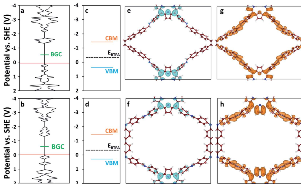
Fig. 2 Density of states (DOS) of (a) RICE-1 and (b) RICE-2. The horizontal axis of (a–d) has units of states \text{eV}^{-1} \text{cell}^{-1} . The red lines represent the highest occupied energy level and the green lines represent the position of the calculated BGC. Band diagrams of (c) RICE-1 and (d) RICE-2 were calculated from the BGC in (a) and (b), respectively, combined with the experimentally measured bandgap using eqn (S1) and (S2).† Orange, blue, and black-dashed lines represent CBM, VBM, and the position of BTTPA redox potential ( E_{\text{BTTPA}} ), respectively. 23 The orbital images of the VB edge (blue isosurfaces) of (e) RICE-1 (potential range: 0.45 V SHE to -0.01 V SHE in (a)) and (f) RICE-2 (potential range: 0.19 V SHE to -0.13 V SHE in (b)). The orbital images of the CB edge (orange isosurfaces) of (g) RICE-1 (potential range: -1.06 V SHE to -1.37 V SHE in (a)) and (h) RICE-2 (potential range: -1.05 V SHE to -1.39 V SHE in (b)). An isosurface level of 0.005 e Å -3 was used to generate the orbital images. C, N, and H are represented as brown, blue, and white spheres, respectively.
