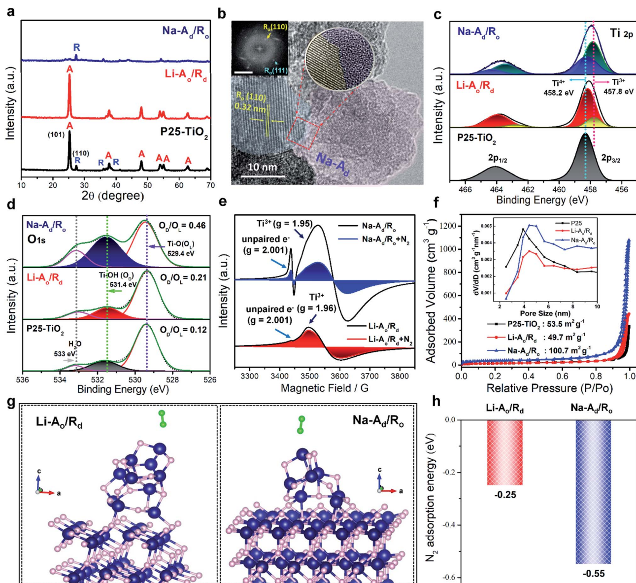
Fig. 2 Structural characterization and simulation for \text{N}_2 adsorption on \text{P25-TiO}_2 , \text{Li-A}_o/\text{R}_d , and \text{Na-A}_d/\text{R}_o . (a) The powder X-ray diffraction spectra (XRD). (b) HR-TEM image of \text{Na-A}_d/\text{R}_o (inset scale bar: 5 \text{ nm}^{-1} ). XPS spectra of (c) \text{Ti } 2p and (d) \text{O } 1s . (e) Electron paramagnetic resonance (EPR) spectra of \text{Li-A}_o/\text{R}_d and \text{Na-A}_d/\text{R}_o before and after \text{N}_2 saturation at 77 K. (f) \text{N}_2 adsorption–desorption isotherms of \text{P25-TiO}_2 , \text{Li-A}_o/\text{R}_d and \text{Na-A}_d/\text{R}_o (inset, corresponding pore-size distribution). (g) Optimized atomic models with \text{N}_2 molecules on \text{Li-A}_o/\text{R}_d and \text{Na-A}_d/\text{R}_o . (h) \text{N}_2 adsorption energy of \text{Li-A}_o/\text{R}_d and \text{Na-A}_d/\text{R}_o . Navy, pink, light green balls represent titanium, oxygen, and nitrogen, respectively.
