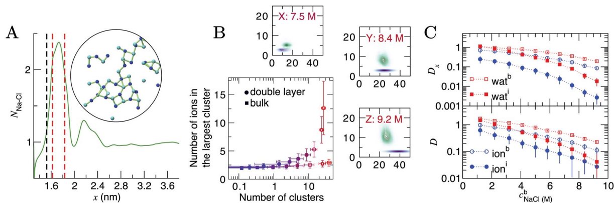
Fig. 5 Ion assembly and diffusion in the double layer. (A) Average Na–Cl first-sphere coordination number ( N_{\text{Na-Cl}} ) as a function of x calculated from a \mu\text{MD} simulation where c_{\text{NaCl}}^{\text{b}} = 9.2 M. The black and red dashed lines indicate the maximum first Na and first two Cl densities in the concentration profiles for Na and Cl highlighted in Fig. 1. Inset is a configuration of a particularly large ionic network identified within the red dashed lines in x . The image is projected onto the yz plane; blue and cyan spheres represent \text{Na}^+ and \text{Cl}^- ions and the green lines highlight ions that are directly coordinated. (B) Ion clusters observed in the bulk and double layer regions of simulations. The blue \rightarrow red colour scale in the main plot indicates increasing c_{\text{NaCl}}^{\text{b}} from 1.2 to 9.2 M. The surrounding panels show purple and green probability densities in the same 2D space for clusters in the bulk and in the double layer, respectively, at the highest bulk concentrations shown by the legend. (C) Diffusion coefficients, D , for ions and water in 0.4 nm regions at the interface and in the bulk region of \mu\text{MD} simulations (indicated by the subscripts i and b in the legends). The top panel provides the x component of D . Data have been scaled by 1 \times 10^{-5} \text{ cm}^2 \text{ s}^{-1} and error bars show uncertainties of one standard deviation.
