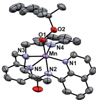
Fig. 6 ORTEP diagram of cationic portion of [\text{Mn}^{\text{III}}(\text{OOCm})(^{\text{6Me}}\text{dpaq})](\text{OTf}) showing 50% probability thermal ellipsoids. Hydrogen atoms of the ^{\text{6Me}}\text{dpaq} ligand, solvent of crystallization, and the triflate counterion were omitted for clarity.
