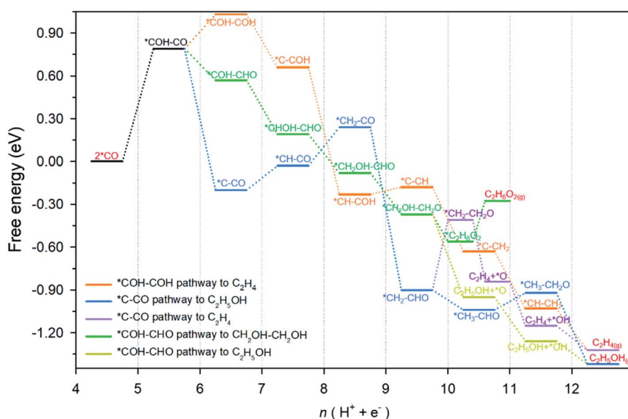
Fig. 2 Reaction pathways and free energy for each state identified on Cu-DAN. The reaction pathway from \text{CO}_2 or \text{CO} to ^*CO adsorption is not shown. The reference energy level is set to be two ^*CO adsorption at 0 V vs. reversible hydrogen electrode (RHE). Pathways toward \text{C}_2 products (ethylene, ethanol and ethylene glycol) beyond 2 ^*CO are shown as different colored branches: orange, ^*COH-COH pathway toward \text{C}_2\text{H}_4 , blue, ^*C-CO pathway toward \text{C}_2\text{H}_5\text{OH} , purple, ^*C-CO pathway bifurcating to \text{C}_2\text{H}_4 , green, ^*COH-CHO pathway toward \text{C}_2\text{H}_6\text{O}_2 and, brown, ^*COH-CHO pathway bifurcating to \text{C}_2\text{H}_5\text{OH} .
