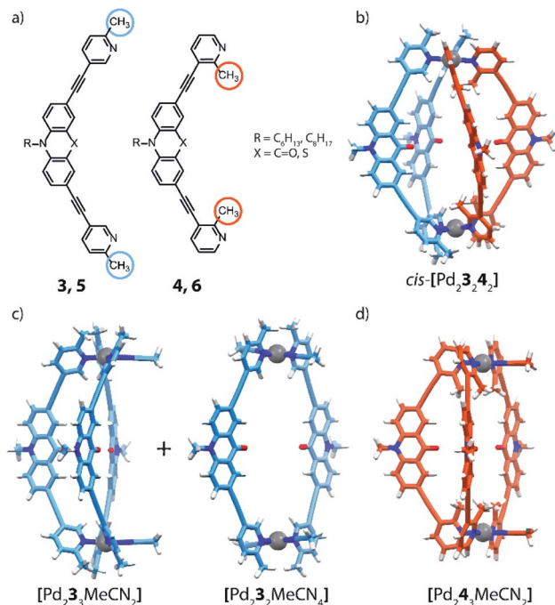
Fig. 5 (a) Banana-shaped ligands with outside- and inside-pointing methyl groups; (b) DFT model of heteroleptic cage cis -[Pd 2 L 3.2 L 4.2 ]; (c) DFT model of bowl and ring obtained with ligand 3 and (d) bowl obtained with ligand 4 .
