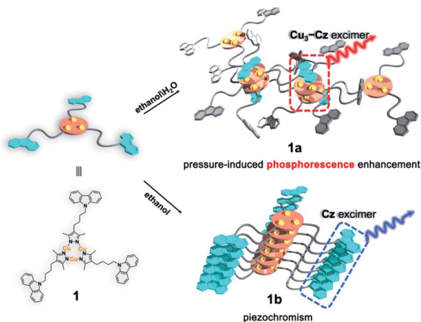
Scheme 1 A schematic representation showing the molecular stacking of two crystalline polymorphs 1a and 1b , and the formation of the Cu 3 Pz 3 CTC Cz–Cu 3 –Cu 3 –Cz excimer and carbazole (Cz) excimer/aggregator, respectively (Scheme 1). Therefore, metal-sensitized phosphorescence and the ligand-dominated luminescence are observed for 1a and 1b , respectively. Furthermore, 1a shows an unprecedented PIPE phenomenon, which has never been reported in piezochromic materials, and 1b exhibits conventional carbazole characteristic piezochromic luminescence with a good linear relationship of intensity versus external pressure.
