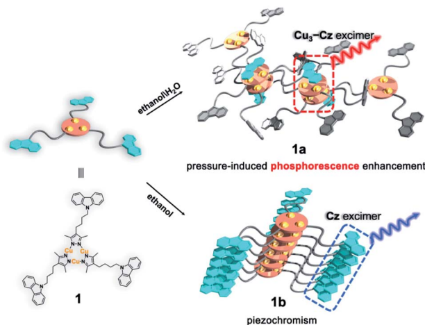
Scheme 1 A schematic representation showing the molecular stacking of two crystalline polymorphs 1a and 1b , and the formation of the \text{Cu}_3\text{Pz}_3 CTC \text{Cz}-\text{Cu}_3-\text{Cu}_3-\text{Cz} excimer and carbazole (Cz) excimer with an increase in pressure.
