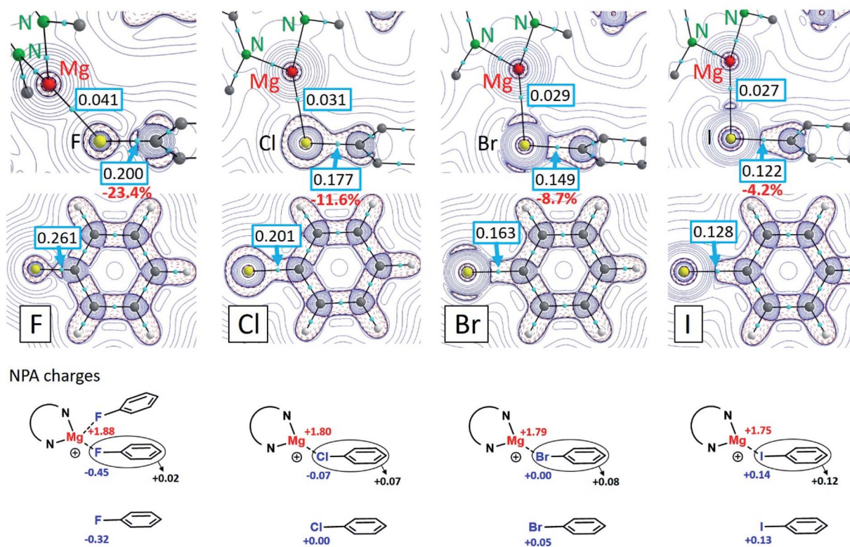
Fig. 3 Contour plots of the negative Laplacian, -\nabla^2\rho(r) , for the cations (t^{\text{Bu}}\text{BDI})\text{Mg}^+\cdots\text{XPh} (X = F, Cl, Br, I) in the \text{Mg}\cdots\text{X-C} plane (top row) and for the free halobenzenes PhX in the molecule plane (middle row). Light-blue dots are bond-critical-points (BCP) and boxed numbers show the electron densities in these points. NPA charges are shown in the bottom part.
