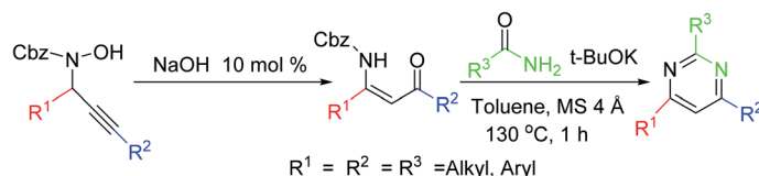
Scheme 10 Pyrimidine synthesis via stereoselective access to β-enaminones.
