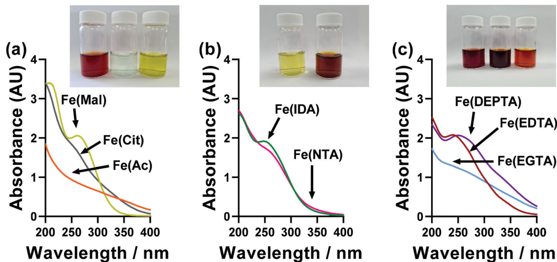
Fig. 6 UV-Vis spectroscopic absorption spectra of the semi-optimized Fe(ligand) systems, using only 2.5 mM Fe(III) and a 1 mm pathlength. The data for Fe(II) and Fe(III) solutions can be found in Fig. S6†. The inset photographs in each figure are for the 100 mM solutions used in the thermogalvanic measurements, from left to right; Fe(Ac), Fe(Mal), Fe(Cit), Fe(IDA), Fe(NTA), Fe(EDTA), Fe(EGTA) and Fe(DEPTA).
