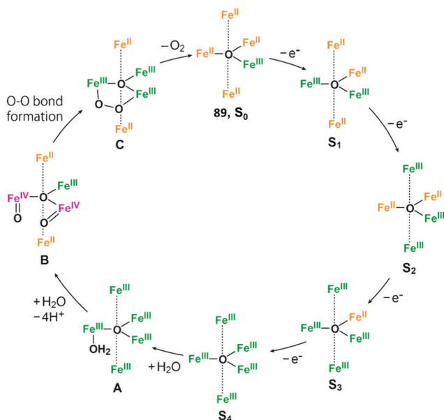
Fig. 40 Plausible catalytic cycle water oxidation promoted by the pentairon complex 89 .
