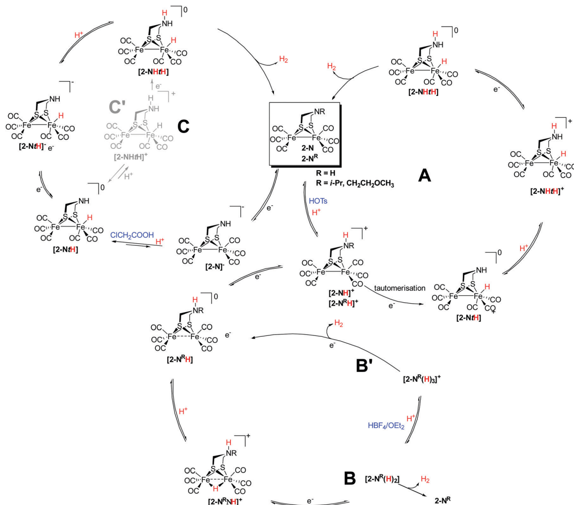
Fig. 99 Catalytic pathways for the proton reduction by \text{Fe}_2(\text{adn})(\text{CO})_6 and \text{Fe}_2(\text{adn}^R)(\text{CO})_6 analogues with acids of varying strength.
