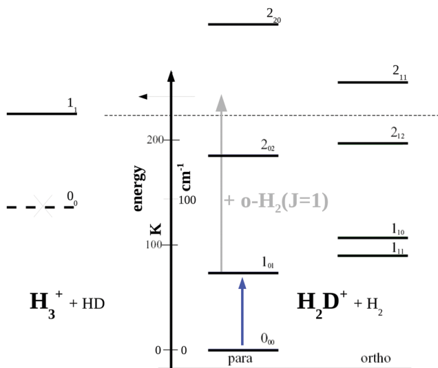
Fig. 5 Rotational levels involved in the low-temperature reaction \text{H}_2\text{D}^+ + \text{H}_2 \rightarrow \text{H}_3^+ + \text{HD} (reaction (R1)). The lowest level of \text{H}_3^+ is 1_1 as the level 0_0 is forbidden by Pauli exclusion. The given endothermicity (thin dashed line at 232 K) is the difference between the lowest rotational levels of the reactant \text{H}_2\text{D}^+ ( 0_{00} ) and product \text{H}_3^+ ( 1_1 ). The energy scale is given in K as well as \text{cm}^{-1} ( 1 \text{ cm}^{-1} \approx 1.4388 \text{ K} ). A similar Figure can be found in ref. 83.
