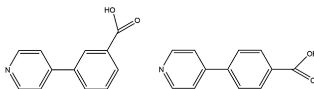
Scheme 1 3-(Pyridin-4-yl)benzoic acid (H34pba) and 4-(pyridin-4-yl)benzoic acid (H44pba).
