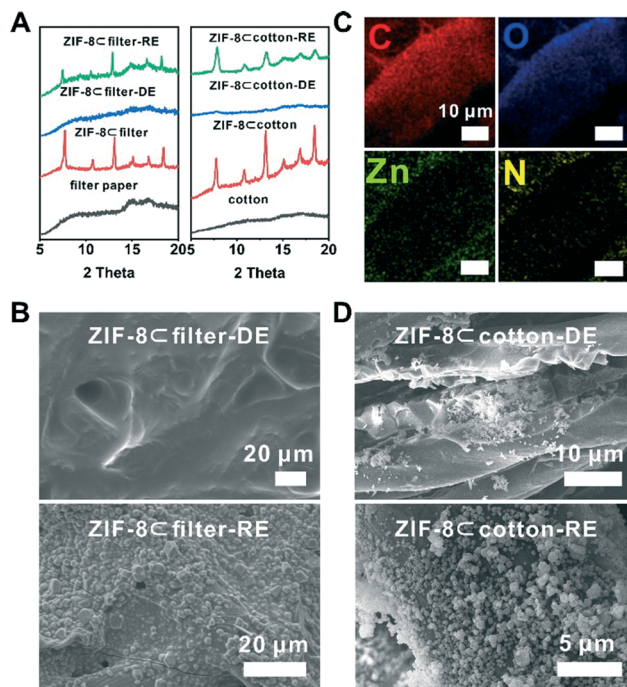
Fig. 3 (A) PXRD patterns of the degradation–reconstruction processes of ZIF-8 on filter and ZIF-8 on cotton; SEM images of (B) ZIF-8 on filter after degradation and reconstruction and (D) ZIF-8 on cotton after degradation and reconstruction; (C) EDS elemental mapping images of ZIF-8 on filter after degradation.
