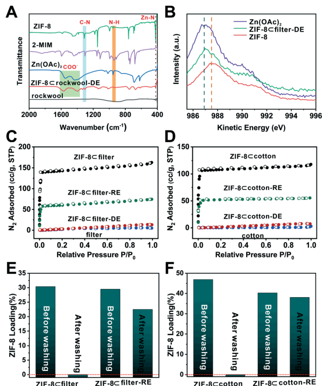
Fig. 4 (A) The FTIR spectrum of ZIF-8, 2-MIM, \text{Zn}(\text{OAc})_2 , ZIF-8 on rockwool-DE and rockwool. (B) The Zn LMM Auger spectrum of \text{Zn}(\text{OAc})_2 , ZIF-8 on filter-DE and ZIF-8; 77 K \text{N}_2 sorption isotherms of (C) ZIF-8 on filter and (D) ZIF-8 on cotton during the degradation–reconstruction cycle; ZIF-8 loading of (E) ZIF-8 on filter and ZIF-8 on filter-RE before and after washing and (F) ZIF-8 on cotton and ZIF-8 on cotton-RE before and after washing.
