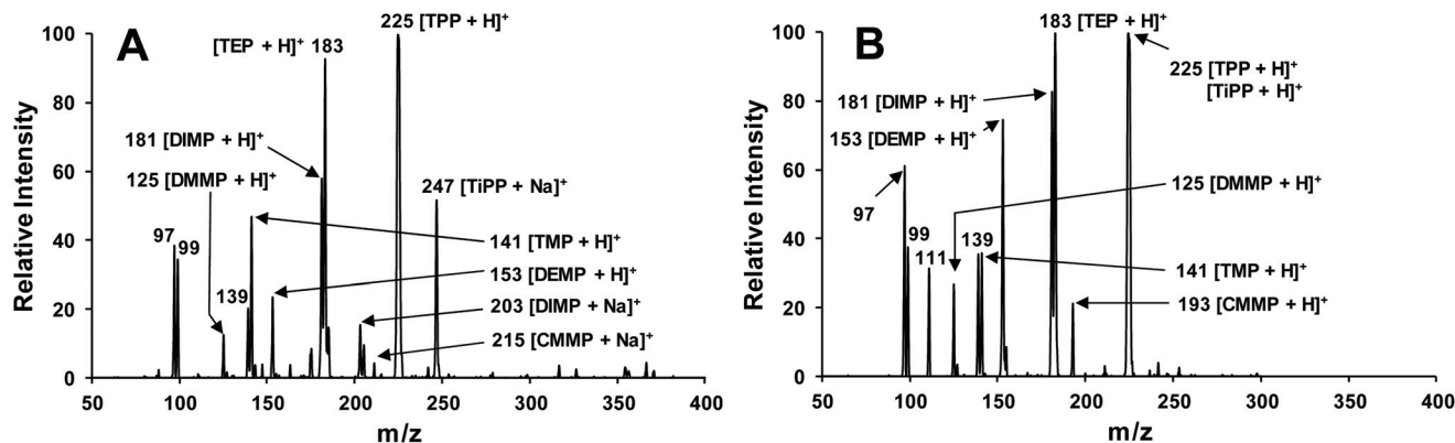
Fig. 3 3D-PCSI-MS collected on the portable AI-MS from a mixture of DMMP, TMP, DEMP, DIMP, TEPP, CMMP, TPP, and TiPP (all at 5 ppm each) in sand. Spectra (A) collected at 1 min of analysis time yield both protonated and sodiated adducts for some target CWA simulants, where spectra (B) from ~7 min predominately show only the protonated forms, as salt leaves the sand matrix.
