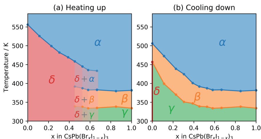
Fig. 4 (a) Heating phase diagram for \text{CsPb}(\text{Br}_x\text{I}_{1-x})_3 thin films aged in a humid environment for composition, x , between 0 (pure \text{CsPbI}_3 ) and 1 (pure \text{CsPbBr}_3 ), where \delta refers to the non-perovskite orthorhombic phase, \alpha is the cubic, \beta is the tetragonal, and \gamma is the orthorhombic perovskite phase. (b) Cooling phase diagram for the same \text{CsPb}(\text{Br}_x\text{I}_{1-x})_3 thin films as they cool down from a high temperature. For the pure \text{CsPbI}_3 thin film, cooling down in nitrogen atmosphere at 2.5 \text{ K min}^{-1} leads to a conversion into the \delta -phase, as marked with a red dot.
