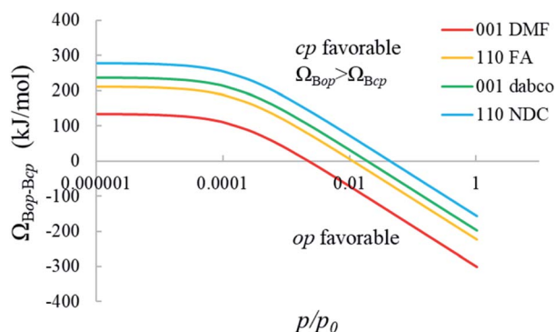
Fig. 10 Relative osmotic potentials, \Omega_{\text{Bop-Bcp}} in the slab models with different capping groups as function of pressure. The gate closing pressure can be found at \Omega_{\text{Bop-Bcp}} = 0 .
