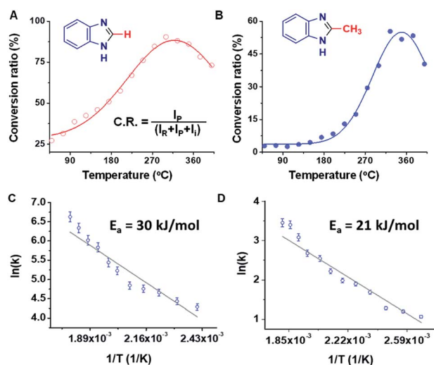
Fig. 2 Effect of inlet temperature of the mass spectrometer on ion intensity, showing conversion ratio (CR) vs. temperature plot for synthesis of (A) benzimidazole and (B) 2-methylbenzimidazole. The equation inset in (A) is used to calculate conversion ratio, where R, P, and I refer to reagent, product and intermediate, respectively. Plots (C) and (D) display temperature-dependent rates plotted against 1/T and give activation energies for the reactions leading to benzimidazole and 2-methylbenzimidazole, respectively.
