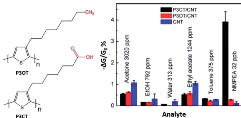
Fig. 21 The chemical structure of P3OT and P3CT, and their responses of the P3CT/CNT, P3OT/CNT sensor, and the non-functionalised CNT sensor to 20 s vapour exposures of various compounds (1% of saturated vapour) and 32 ppb of NMPEA. Reproduced from ref. 201, copyright 2018, Elsevier.
