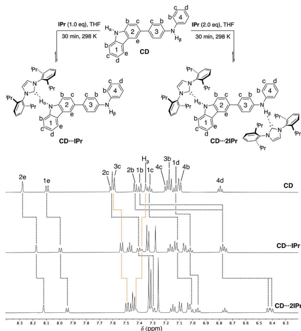
Fig. 6 Partial ^1\text{H} NMR spectra (500 MHz, \text{THF-}d_8 ) of CD (50 mM), CD...IPr, and CD...2IPr, highlighting the chemical shift changes upon hydrogen bonding to IPr. CD \text{H}_z (10.25 ppm), CD...IPr \text{H}_z (11.30 ppm), and CD...2IPr \text{H}_z (12.40 ppm) are broadened due to exchange, see ESI† (rings 1 and 2 = black dotted lines, rings 3 and 4 = orange dotted lines).
