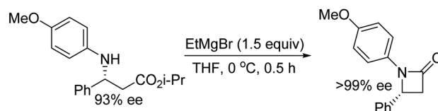
Fig. 58 CPA catalysed ATH of \beta -N-substituted enamine esters and construction of chiral \beta -lactam.
