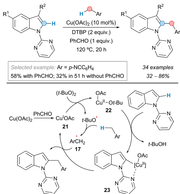
Scheme 12 C2-Benzylation of 1-pyrimidyl-substituted indoles and proposed catalytic cycle.
