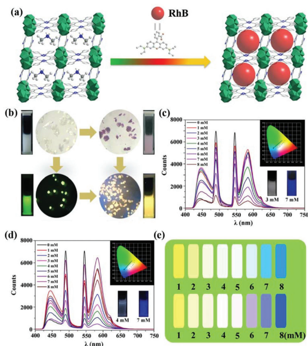
Fig. 16 (a) The 3D porous anion framework of Tb-dcppt and the fabrication of RhB@Tb-dcppt via cation exchange. (b) Photographs of both samples under natural light and UV lamp at 365 nm. Emission spectra of the RhB@Tb-dcppt aqueous suspension upon various concentrations of (c) NFX and (d) CPFX. (e) The corresponding luminescence colours. Reproduced from ref. 117 with permission from the American Chemical Society.
