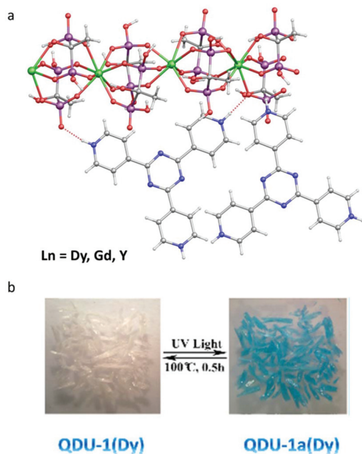
Fig. 2 (a) Crystal structures of QDU-1(Ln) ; (b) reversible photochromic behaviour between QDU-1(Dy) and QDU-1a(Dy) . Reproduced with permission from ref. 43. Copyright 2020 American Chemical Society. 43
