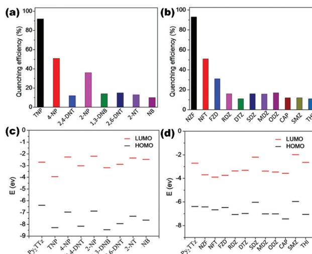
Fig. 5 (a and b) Quenching (%) for (24) upon addition of different NACs and antibiotics; (c and d) Comparisons of HOMO and LUMO energies for linker Py 2 TTz with selected NACs and antibiotics. Reproduced with permission from ref. 80. Copyright 2018 American Chemical Society.
