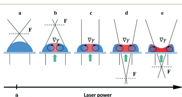
Fig. 2 Schematic illustration of the droplet reshaping by the thermocapillary forces induced with the laser beam. The axis shows the laser power increase. \nabla \gamma is the thermal surface tension gradient along the liquid interface. (a) The initial shape of the droplet (the laser is off); (b) the flattening of the droplet surface – the focal length increases (the laser is on); (c) the droplet with the flat surface – the focal length tends to infinity; (d) and (e) the formation of thermocapillary dimple in the droplet, negative focal length.
