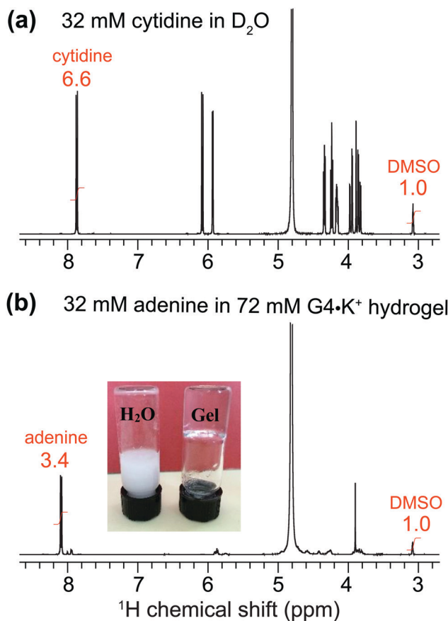
Fig. 4 Solution-state 1D ^1\text{H} (600 MHz) NMR spectrum of (a) 32 mM of cytidine dissolved in D 2 O using DMSO proton signals (at 3.09 ppm, integral of 1.0) as an internal calibration standard, and (b) of 32 mM adenine incorporated into a G4-K + gel. The inset image in (b) depicts the dissolution of 32 mM of adenine in H 2 O (left) and in 72 mM G4-K + borate gel (right).
