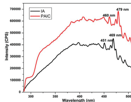
Fig. 5 Crystals of a luminescent CP based on Ca and itaconic acid, and solid state luminescence spectra of the ligand (IA) and CP (PAIC) at room temperature with \lambda_{\text{max}} = 285 \text{ nm} . Reprinted from ref. 67 with permission from Elsevier.
