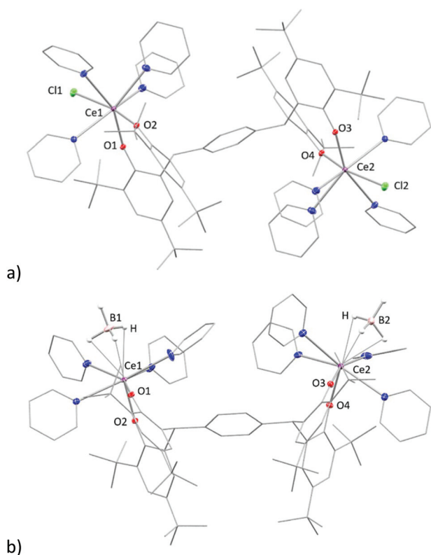
Fig. 3 Solid state structure of complex (a) 3-Ce (b) 3-Ce-BH 4 . Thermal ellipsoids are shown at 30% probability. All hydrogen atoms (except for \text{BH}_4 ) and solvents are omitted for clarity. Selected bond lengths in (a): Ln1–Cl1: 2.7789(6)\text{ }\text{\AA} (Ce), 2.7601(14)\text{ }\text{\AA} (Pr).
