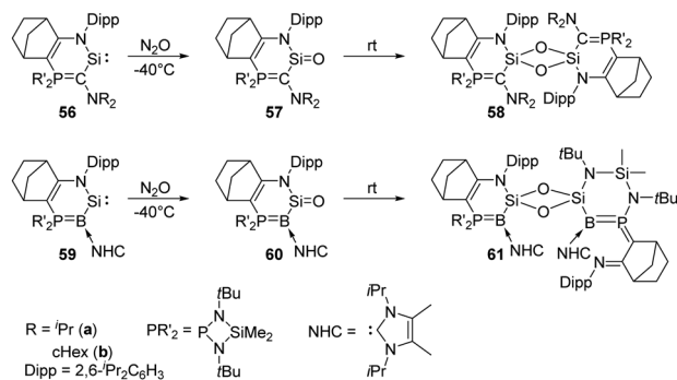
Scheme 22 Oxygenation of the phosphonium ylide and phosphonium bora-ylide silylenes 56 and 59 by N_2O .
