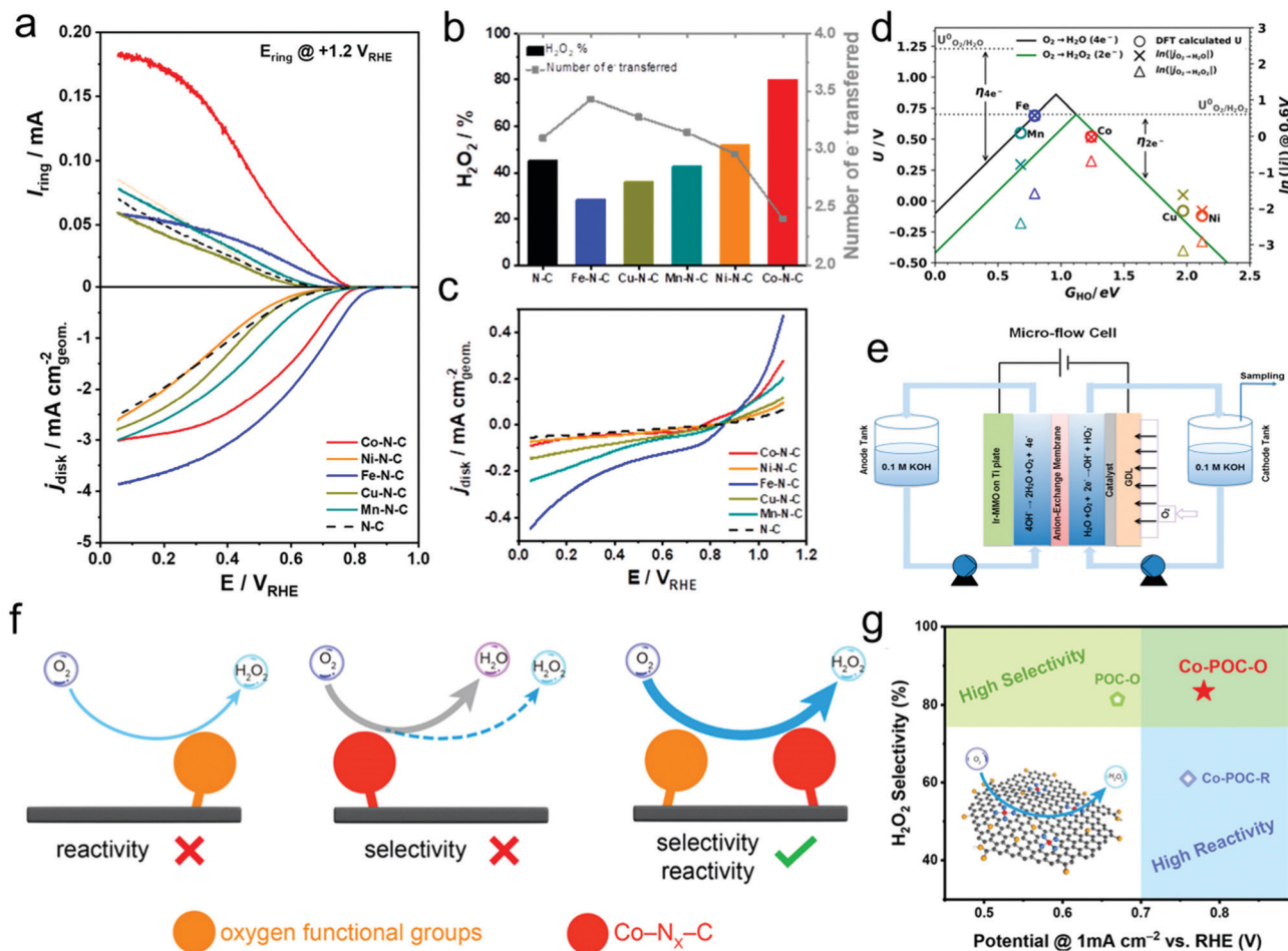
Fig. 3 (a) Linear sweep voltammetry (LSV) in a rotating ring-disk electrode (RRDE) setup with the Pt ring held at +1.2 \text{ V}_{\text{RHE}} . (b) H 2 O 2 selectivity (H 2 O 2 %) and the number of electrons ( n ) at +0.1 \text{ V}_{\text{RHE}} derived from RRDE data. (c) Background-corrected H 2 O 2 RR performance in N 2 -saturated 0.5 M H 2 SO 4 electrolyte containing 1 mM H 2 O 2 . (d) Thermodynamic relations (volcano) lines for the two- (green solid line) and four- (black solid line) electron ORR. The DFT calculated ORR onset potential values (circles) are on the left y-axis, while the experimental current densities (crosses and triangles), reported as \ln(|j|) , are on the right y-axis. Both are shown as functions of the chosen reaction descriptor, the DFT calculated HO* binding free energy ( G_{\text{HO}} ). (e) Scheme of the micro-flow cell setup. (f) Mechanism of the synergistic strategy of atomic Co-N x -C sites and OFGs for H 2 O 2 electrocatalysis on noble-metal-free electrocatalysts. (g) Performance comparison in regard to reactivity and selectivity for H 2 O 2 electrocatalysis on Co-POC-O, Co-POC-R, and POC-O electrocatalysts. The inset in (g) shows the mechanism scheme for synergistic H 2 O 2 electrocatalysis. The carbon, nitrogen, oxygen, and cobalt atoms are marked with black, blue, yellow, and red, respectively. (a–e) Reprinted with permission. 18 Copyright 2019, American Chemical Society. (f and g) Reprinted with permission. 89 Copyright 2019, Wiley-VCH.
