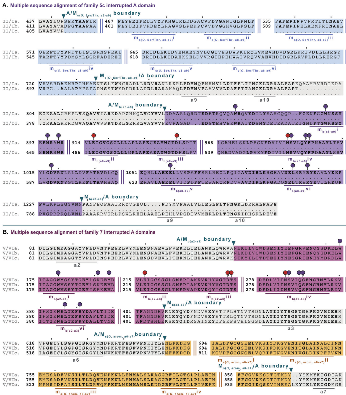
Fig. 10 Multiple sequence alignments of (A) family 5c interrupted A domain (sequence “a”) alignment with representative type II and type I M domains, KtzH(M II ) 4 (sequence “b”) and TiO 2 (M I ) 4 (sequence “c”), respectively, and (B) family 7 interrupted A domains. The A domain is highlighted in light grey and conserved A domain motifs are underlined in dark grey. The M II is highlighted in light blue and the conserved motifs are underlined in dark blue. The M I is highlighted in light purple, and the conserved motifs are underlined in dark purple. The red and dark purple balloons in panel A correspond to residues involved in SAM and amino acid bound Ppant arm binding, respectively, according to the structure of TiO 2 (A 8 M 1 A 9 ) 4 . 14 The identical corresponding residues in type V M domain are also indicated in the same way. Type V M domain is highlighted in light pink and the conserved motifs are underlined in dark pink. Type VI M domain portion is highlighted in light orange and the conserved M domain motifs are underlined in dark orange. The boundaries between the domains are indicated by a triangle. Breaks in the sequences are indicated by two parallel bars. The full sequence alignments and accession numbers are presented in Fig. S19 and S21 (ESI†).
