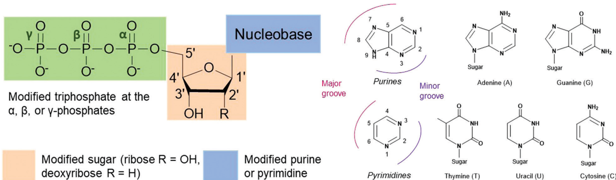
Fig. 1 Possible sites of modification on nucleoside triphosphates (NTPs) to study bacterial cellular processes. Modifications are found on the nucleobase (purines A and G or pyrimidines T, U and C), the sugar moiety (ribose or deoxyribose) or the triphosphate tail ( \alpha -, \beta - or \gamma -position).
