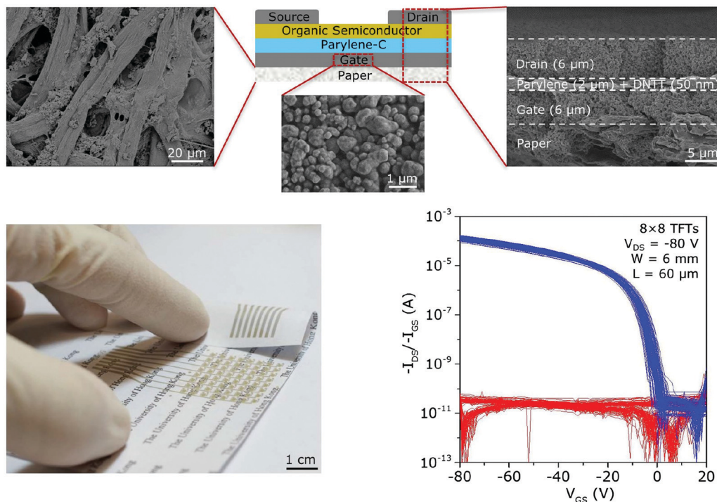
Fig. 2 Array of organic TFTs fabricated by Peng et al. on commercially available laser-printing paper using screen-printed silver-nanoparticle-based gate electrodes and source/drain contacts, a 2 μm-thick vapor-deposited parylene gate dielectric and vacuum-deposited DNNT as the semiconductor. The TFTs have an average carrier mobility of 0.45 \text{ cm}^2 \text{ V}^{-1} \text{ s}^{-1} , and average on/off current ratio of 10^8 , a subthreshold slope of 0.9 V per decade and a transit frequency of 50 kHz. Reprinted with permission. 29 Copyright 2014, Nature Publishing Group.
